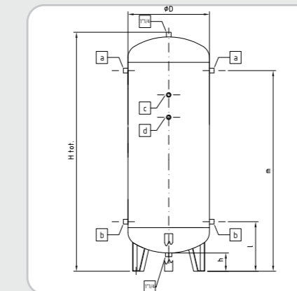
Serbatoio/Vessel CE 2009/105 (ex 87/404)
